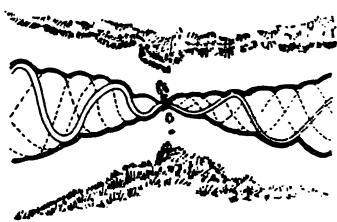
FIG. 183. — Plan of a river narrows.
